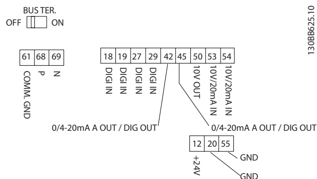
Illustration 1.5 Control Terminals
