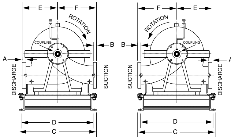
Clockwise Rotation Viewed from the Motor End
