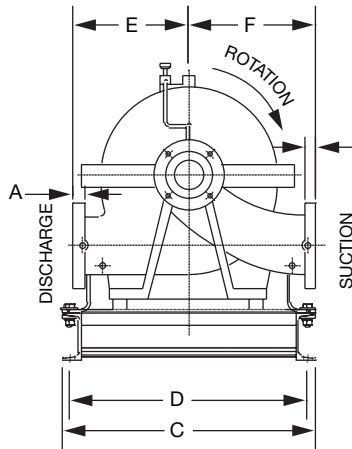
Clockwise Rotation viewed from the Coupling End
