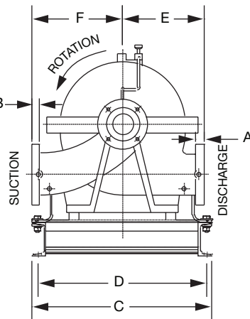
Counterclockwise Rotation viewed from the Coupling End
