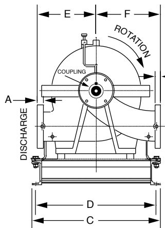
Clockwise Rotation Viewed from the Motor End (motor not shown)
