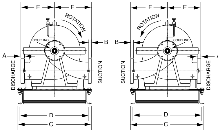
Clockwise Rotation Viewed from the Motor End (motor not shown)
