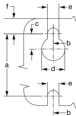
Frames A2 through C2 (4x mounts)
