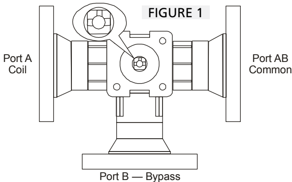
Figure 1: STM Series Three-Way Ball Valve (Coil Port A Open to Common Port AB)
