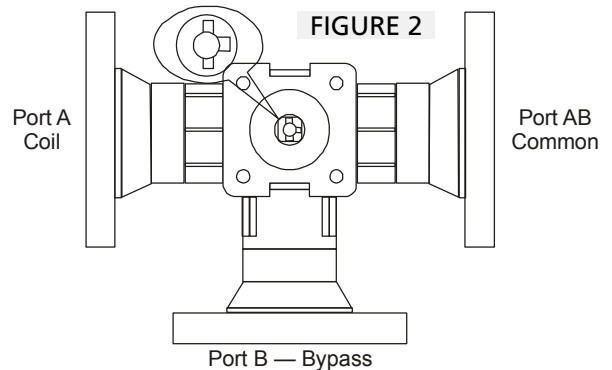
Figure 2: STM Series Three-Way Ball Valve (Bypass Port B Open to Common Port AB)
