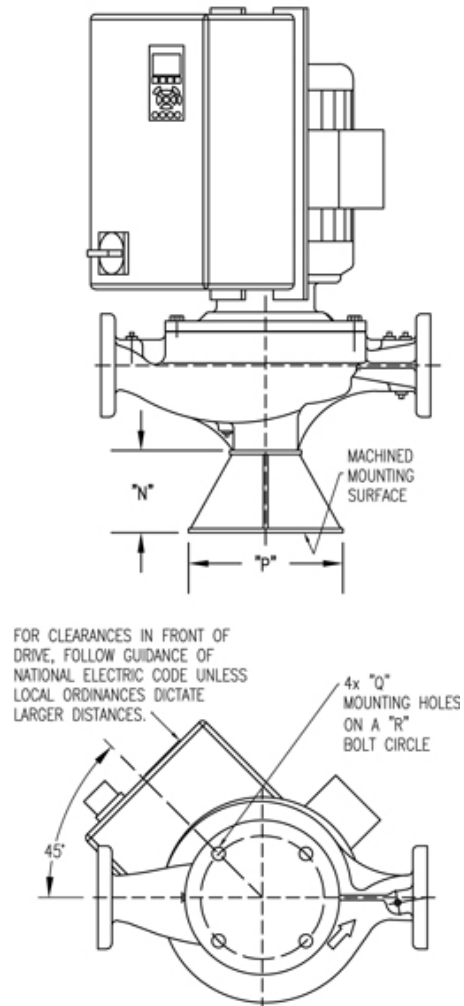
PUMP WITH OPTIONAL SUPPORT STAND
