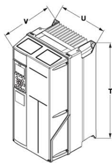
Basic drive
