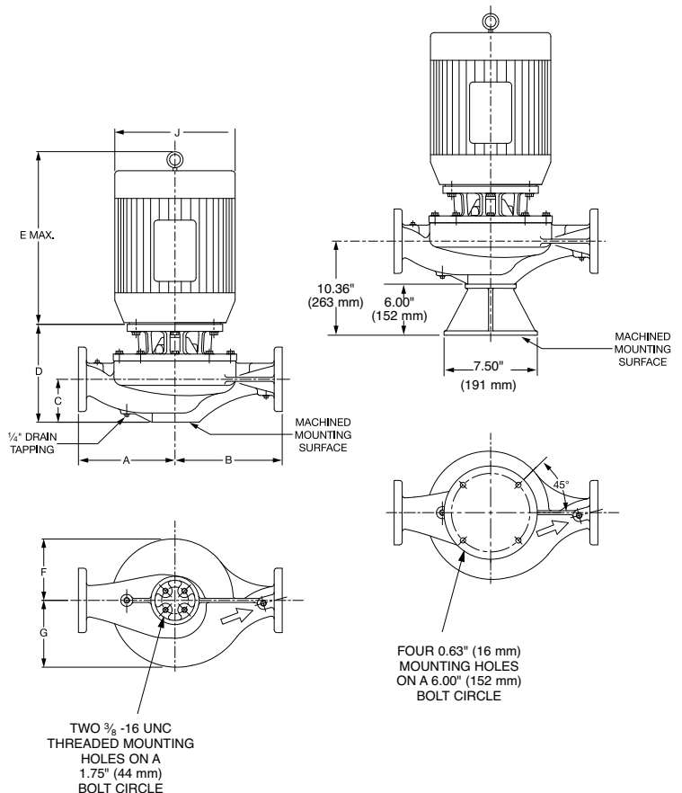
PUMP WITH OPTIONAL SUPPORT STAND
