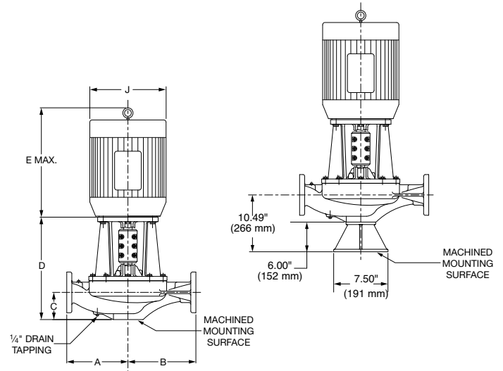
PUMP WITH OPTIONAL SUPPORT STAND
