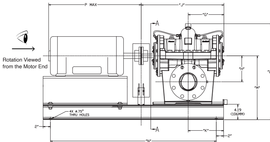
Clockwise Rotation Viewed from the Motor End (motor not shown)
