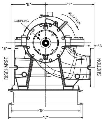
Clockwise Rotation Viewed from the Motor End (motor not shown)
