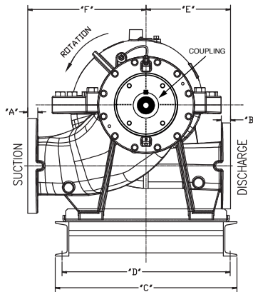
Counterclockwise Rotation Viewed from the Motor End (motor not shown)
