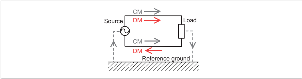
Fig. 5.3 Common-mode and differential-mode
