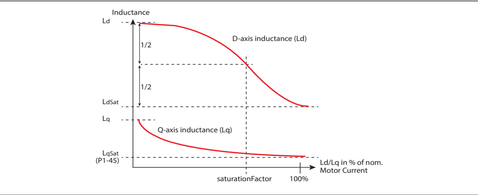
Fig. 1.32 Example of L_d/L_q relationship to I_d/I_q
