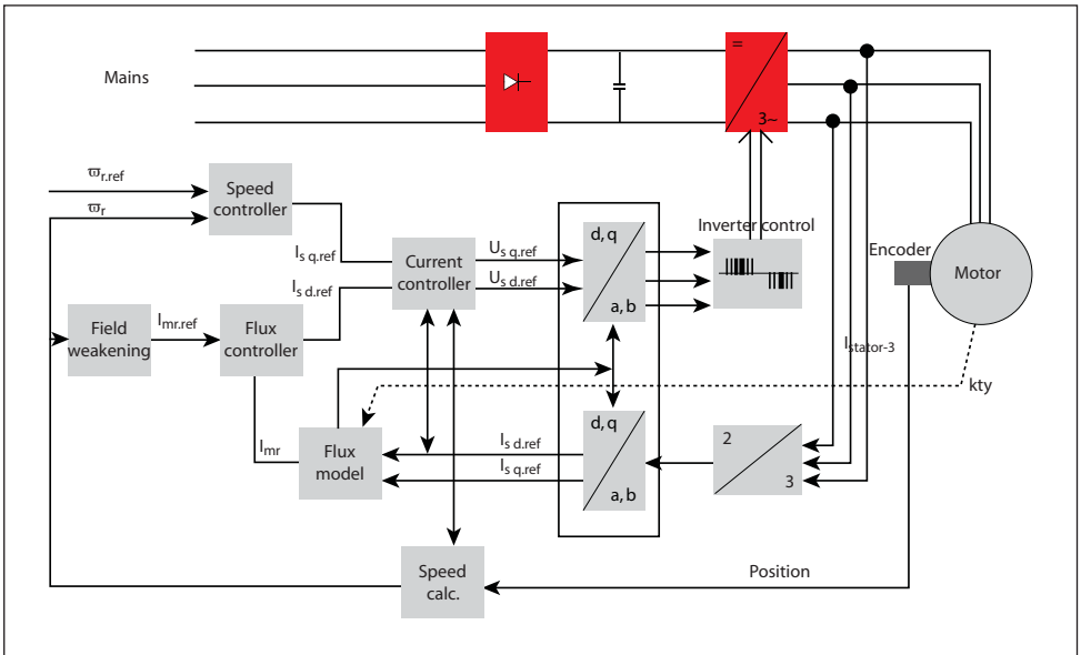
Fig. 2.23 Structure closed loop flux vector control
