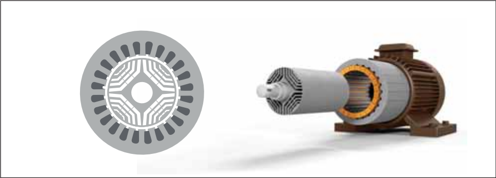
Fig. 1.31 Special rotor lamination design results in high efficiency at low torque ripples
