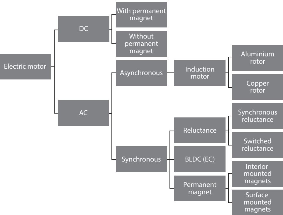
Fig. 1.1 Overview of the most common electric motor technologies
