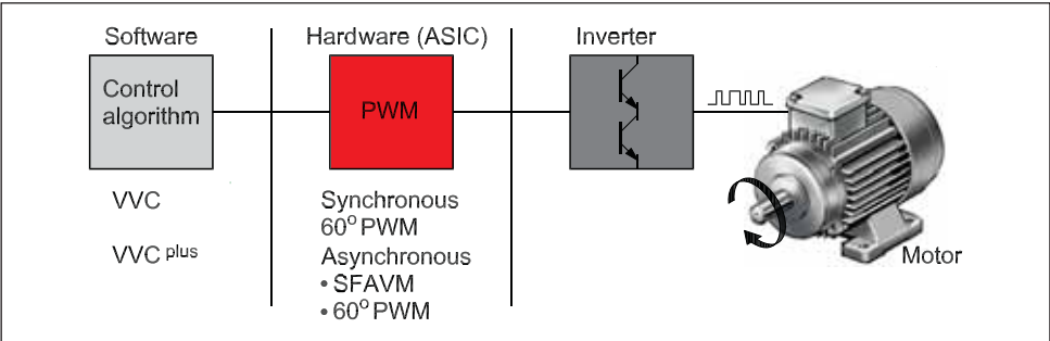
Fig 2.24 Basic principles of current standard frequency converters from Danfoss
