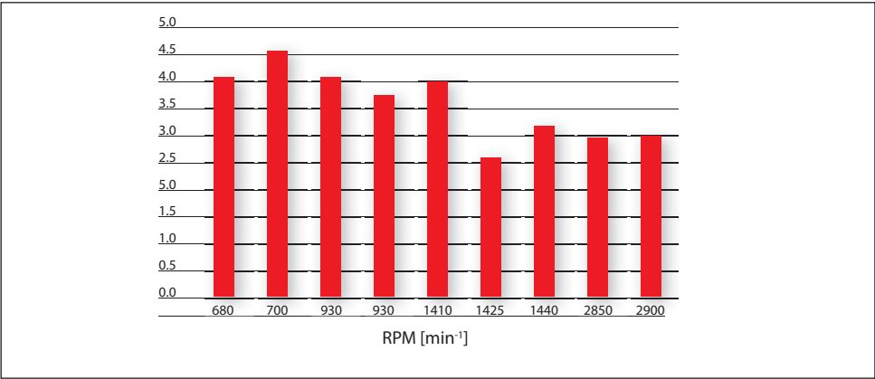
Fig. 9.1 Nominal current for 1.5kW motors of different poles and manufacturer
