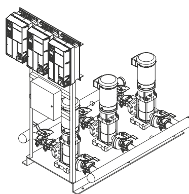
Triplex Booster System
