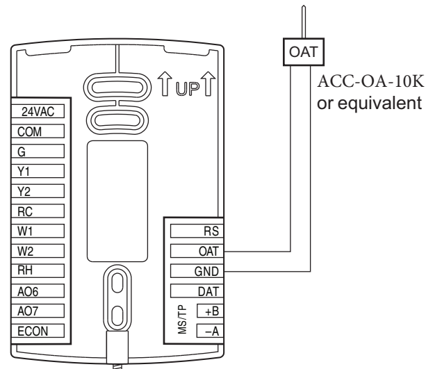
Illustration 2–7 Wiring for an outside air temperature sensor
