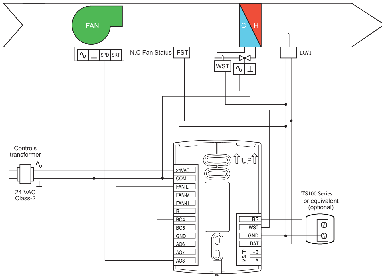
Illustration 6–7 Wiring details: Two-pipe FCU with modulating fan and on/off valve
