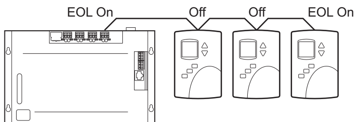
Illustration 7–2 Location for end-of-line termination
