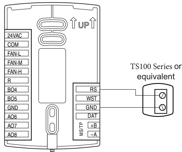
Illustration 2–3 Wiring for remote space temperature sensor
