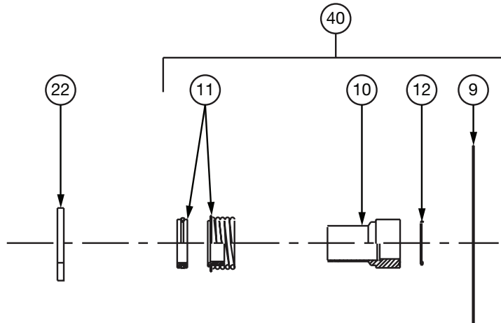
Seal replacement parts
