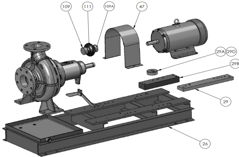
FI 3011 MOTOR FRAMES (NEMA STANDARD) "T"
