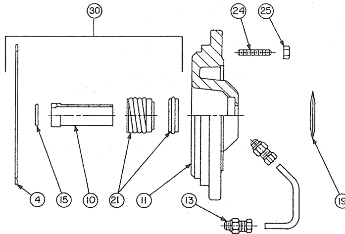
SEAL PARTS FOR VL 2510—SEAL KITS INCLUDE ITEMS NO. 4, 6, 10, 15 &amp; 21
