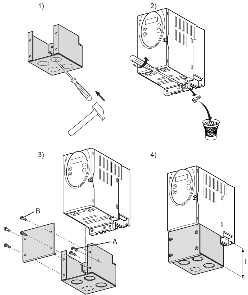
Figure / Figura / Figure 2 : Installation / Instalación / Installation
