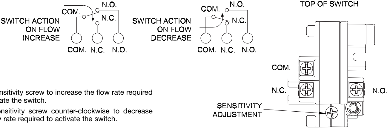
FIG. 6 SWITCH INFORMATION
