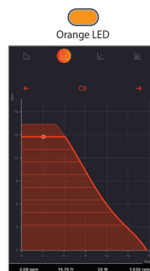
Nine Constant Pressure Curves
