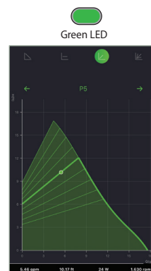
Nine Proportional Pressure Curves
